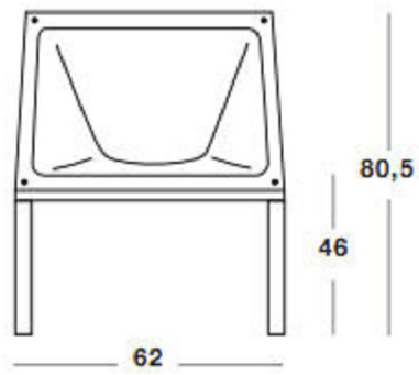
Methacrylate version L 62 P 59 H 80,5 H 46 (seat)
