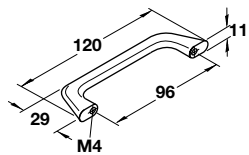
1 - Zinc, matt nickel
